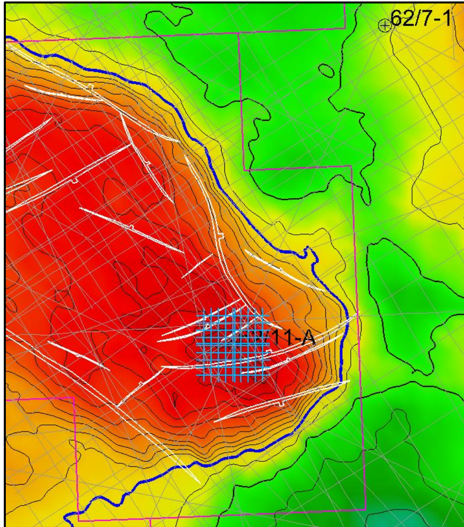
Existing 2D and potential Hi-Res 2D Site Survey
