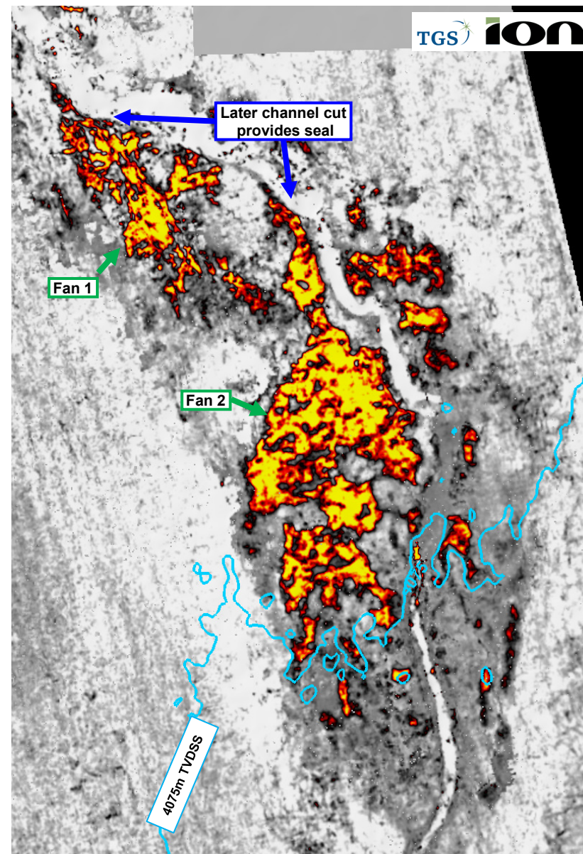
AVO product (Far - Near)*Far
